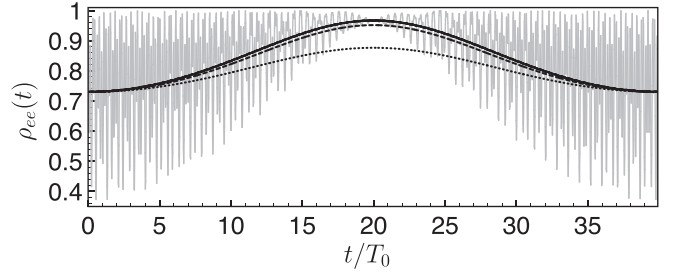
FIG. 5. Higher-order effective master equation vs full quantum evolution. Shown are the instantaneous density-matrix population \rho_{ee}(t) as a function of time (solid gray line, in arbitrary unit T_0 ), time-convoluted population \bar{\rho}_{ex}(t) (solid black line) obtained from the exact unitary evolution, and time coarse-grained density-matrix population \bar{\rho}_{ee}(t) obtained from the second-order (dotted black line) and third-order (dashed black line) effective master equation. Parameters: initial density matrix \rho_0 = |e\rangle\langle e| , constant and fast Hamiltonians \hat{H}_0 = \omega_0 \sigma_z and \hat{H}_F(t) = \Omega[\cos(\omega_1 t) + \cos(\omega_2 t)] \sigma_x . Results obtained for the frequencies: \omega_0 = 0.5 \times (2\pi)/T_0 , \Omega = 3.5/T_0 , and \varepsilon \simeq 0.18 . The frequencies \omega_1 , \omega_2 , and \omega_c are the same as in Figs. 2 and 3 of the main text.
