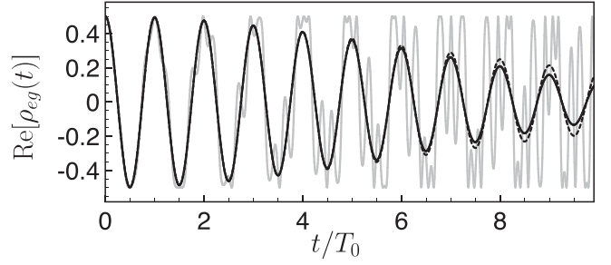
FIG. 2. Emulation of phase noise: results of the effective master equation vs full quantum evolution. Shown are the instantaneous density-matrix coherence \text{Re}[\rho_{eg}(t)] as a function of time (solid gray line), time coarse-grained coherence \text{Re}[\tilde{\rho}_{eg}(t)] (solid black line), and the density-matrix coherence \text{Re}[\tilde{\rho}_{eg}(t)] (dashed black line) obtained from the effective master equation [Eq. (8)]. Parameters: \hat{H}_0 = \omega_0 \sigma_z , \hat{V}_{1,2} = \Omega_{1,2} \sigma_x , \omega_0 = 0.5 \times (2\pi)/T_0 , \Omega_1 = -\Omega_2 = 7/T_0 , \omega_1 = \sqrt{10} \times (2\pi)/T_0 , and \epsilon = 0.35 . Other parameters are identical to Fig. 1.
