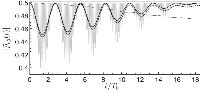
FIG. 1. Quantum dynamics in the interaction picture with \hat{H}_0 = \omega_0 \sigma_z and \hat{V}_{1,2} = \Omega_{1,2} \sigma_x . Shown are the instantaneous density-matrix profile |\tilde{\rho}_{eg}(t)| as a function of time (solid gray line) with \tilde{\rho}(t) = U^{\text{eff}}(t)^\dagger \rho(t) U^{\text{eff}}(t) and coarse-grained density-matrix coherence |\tilde{\rho}_{eg}(t)| as a function of time obtained from a time averaging of the instantaneous solution \tilde{\rho}(t) (solid black line), or from a resolution of the full effective master equation (dashed black line), of an effective master equation without the contribution \mathcal{L}^{FSF}[\tilde{\rho}] (see text) to the quantum dissipation term (dotted line). Parameters: \rho(0) = |\psi_+\rangle\langle\psi_+| where |\psi_+\rangle = (|e\rangle + |g\rangle)/\sqrt{2} , \omega_0 = 0.1 \times (2\pi)/T_0 , \Omega_1 = \Omega_2 = 2/T_0 , \omega_1 = 4 \times (2\pi)/T_0 , \Delta\omega_{21} = 0.025 \times (2\pi)/T_0 , \epsilon = 0.1 .
