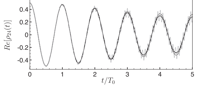
FIG. 4. Emulated decoherence in a harmonic oscillator with \hat{H}_0 = \omega_0 \hat{a}^\dagger \hat{a} and \hat{V}_{1,2} = \pm \Omega \hat{a}^\dagger . Shown are the instantaneous density matrix \text{Re}[\rho_{24}(t)] (solid gray line) and exact TCG density matrix \text{Re}[\bar{\rho}_{24}(t)] (solid black line) elements in the Fock state basis as a function of time compared to the prediction of the effective master equation (dashed black line). Parameters: \omega_1 = 40/T_0 , \Delta\omega_{21} = 0.1 \times (2\pi)/T_0 , \epsilon = \Omega/\omega_1 = 0.15 .
