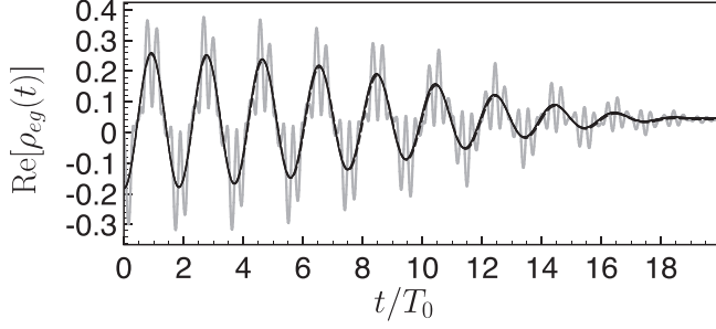
FIG. 3. Incoherent absorption or emission in the time-averaged dynamics. Shown are the instantaneous density-matrix coherence \text{Re}[\rho_{eg}(t)] as a function of time (solid gray line) and time-averaged coherence \text{Re}[\bar{\rho}_{eg}(t)] (solid black line) vs density-matrix coherence \text{Re}[\bar{\rho}_{eg}(t)] (dashed black line) obtained from the effective master equation. Parameters: \hat{H}_0 = \omega_0 \sigma_x , \hat{V}_{1,2} = \Omega_{1,2} \sigma_+ , \rho(0) = |e\rangle\langle e| , \omega_0 = 0.25 \times (2\pi)/T_0 , \Omega_{1,2} = 2/T_0 , \epsilon = 0.1 . Other parameters are identical to Fig. 2.
