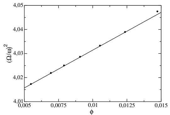
FIG. 3. \left(\frac{\Omega}{\omega}\right)^2 as a function of the dimensionless density, \phi . The dots are the simulation results and the solid line is the theoretical prediction (13).
