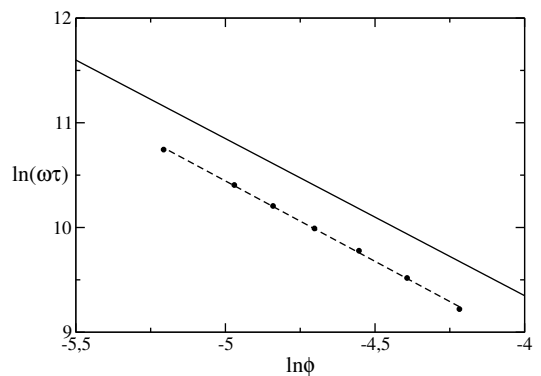
FIG. 4. \omega\tau as a function of the dimensionless density, \phi , in logarithmic scale. The points are the simulation results, the solid line is the theoretical prediction for \tau as defined above (13) and the dashed line is the linear fitting of the simulation results.
