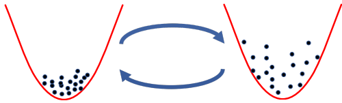
FIG. 1. (Color online) Sketch of the system. The particles, shown with the disks, are confined in the (red) parabolic potential. Under generic initial conditions, the system evolves towards a breathing state, oscillating between a dense configuration with high temperature (left) and a more dilute configuration with a smaller temperature and a higher potential energy (right).
