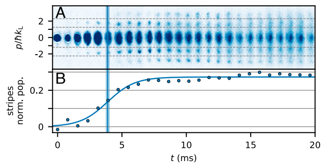
Fig. 5. Long-term survival of the emerging crystal-like order. (A) Experimental stroboscopic evolution of the momentum distribution after band-mapping over 510 periods of modulation. Modulation parameters are s_0 = 3.8 \pm 0.1 , \nu = 25.5 kHz, and \varphi_0 = 15^\circ . The initial growth of the instability is monitored by counting the relative atomic population in the two stripes delimited by dashed lines. (B) Evolution of the normalized population in momentum peaks created by the instability [stripes in (A)]. A sigmoid fit allows us to determine the nucleation timescale t_n \approx 4 ms. The population in the nucleated modes then settles and remains identifiable on a timescale of several t_n , but an eventual broadening of the momentum peaks is clearly visible in (A).
